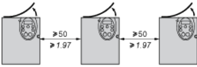
Type C mounting mm in.
